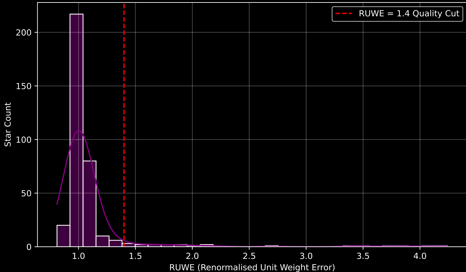
GAPOGEE DR17 Field [281-06] RUWE Distribution (n= 354)
