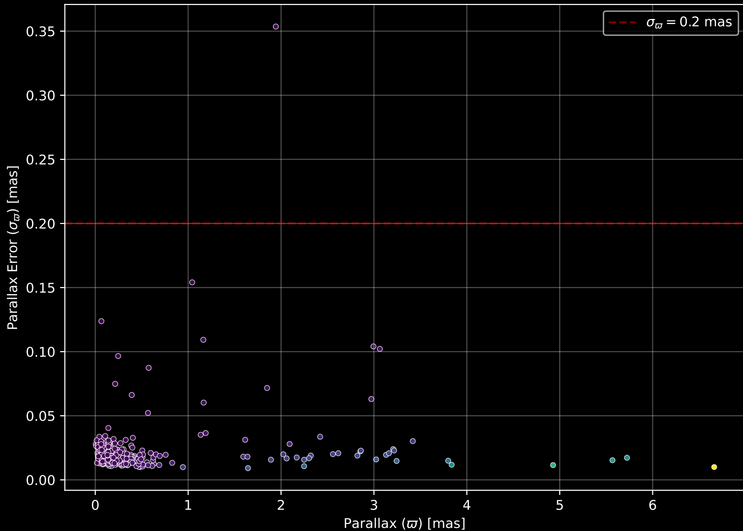
APOGEE DR17 Field: [281-06] Parallax Quality (n= 361)
