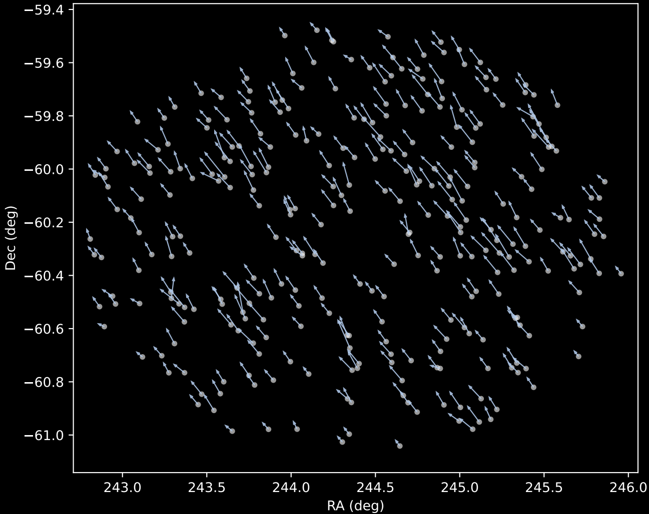
APOGEE DR17 Cluster 1 Proper Motion Vectors (n=305)
